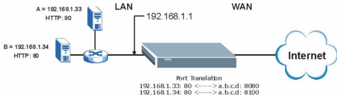
Figure 143 Port Translation Example
