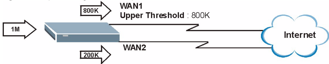
Figure 48 Spillover Algorithm Example
