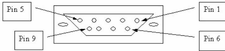
Figure 363 Console/Dial Backup Port Pin Layout
