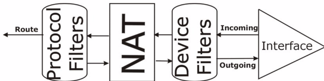
Figure 303 Protocol and Device Filter Sets
