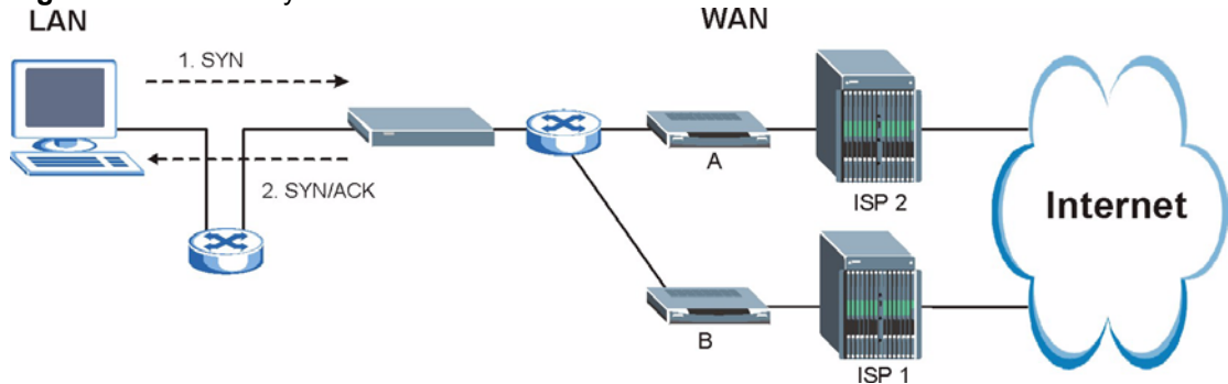
Figure 389 Gateways on the WAN Side
