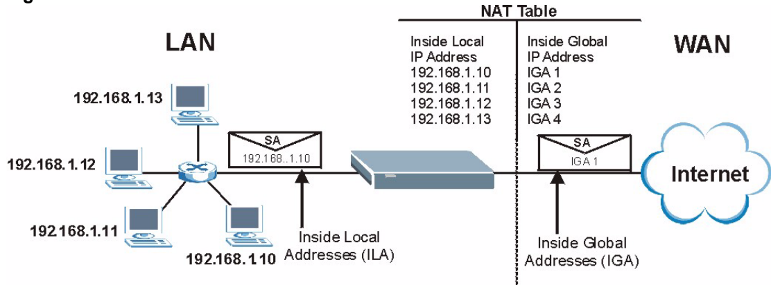
Figure 137 How NAT Works
