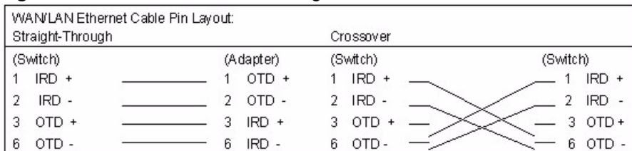
Figure 364 Ethernet Cable Pin Assignments
