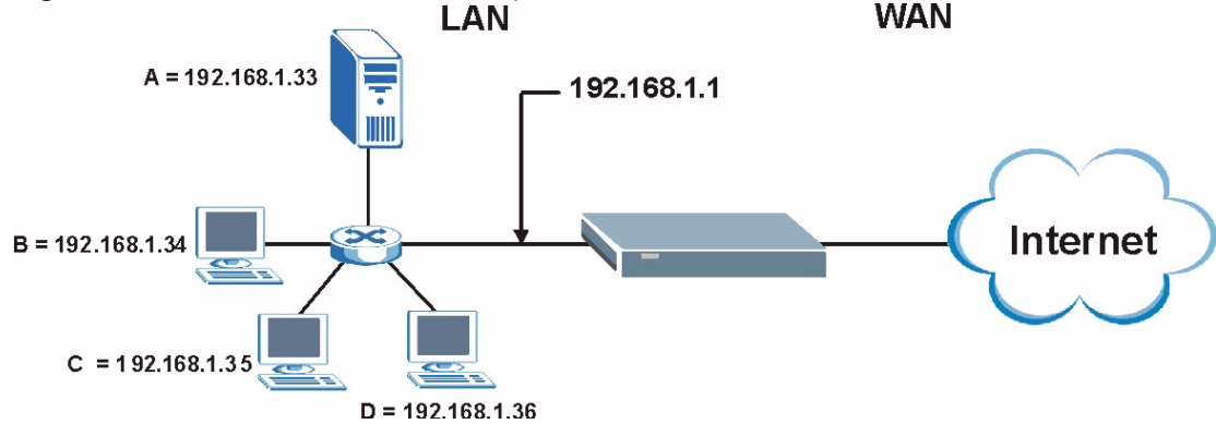
Figure 277 Server Behind NAT Example
