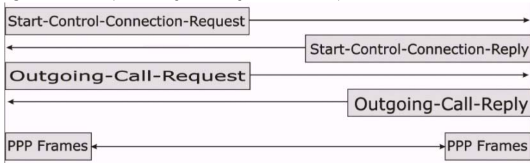
Figure 382 Example Message Exchange between Computer and an ANT
