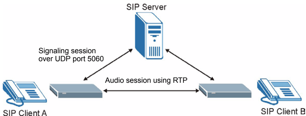
Figure 393 ZyWALL SIP ALG
