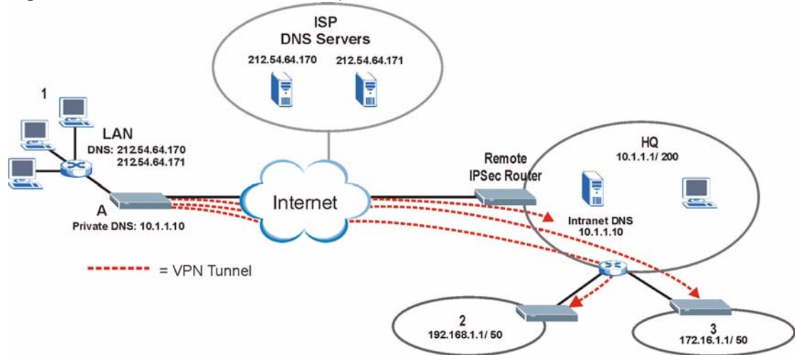
Figure 163 Private DNS Server Example
