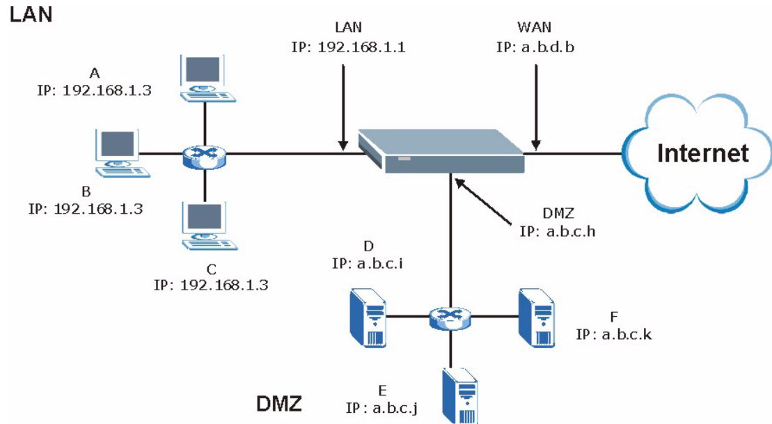
Figure 63 DMZ Public Address Example
