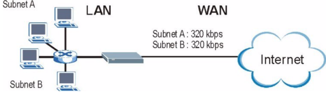
Figure 153 Subnet-based Bandwidth Management Example
