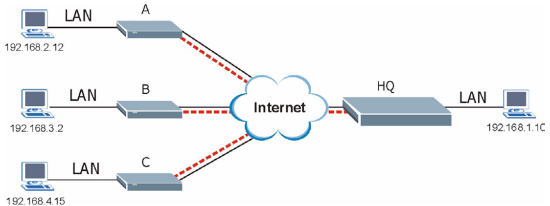
Figure 120 Telecommuters Sharing One VPN Rule Example
