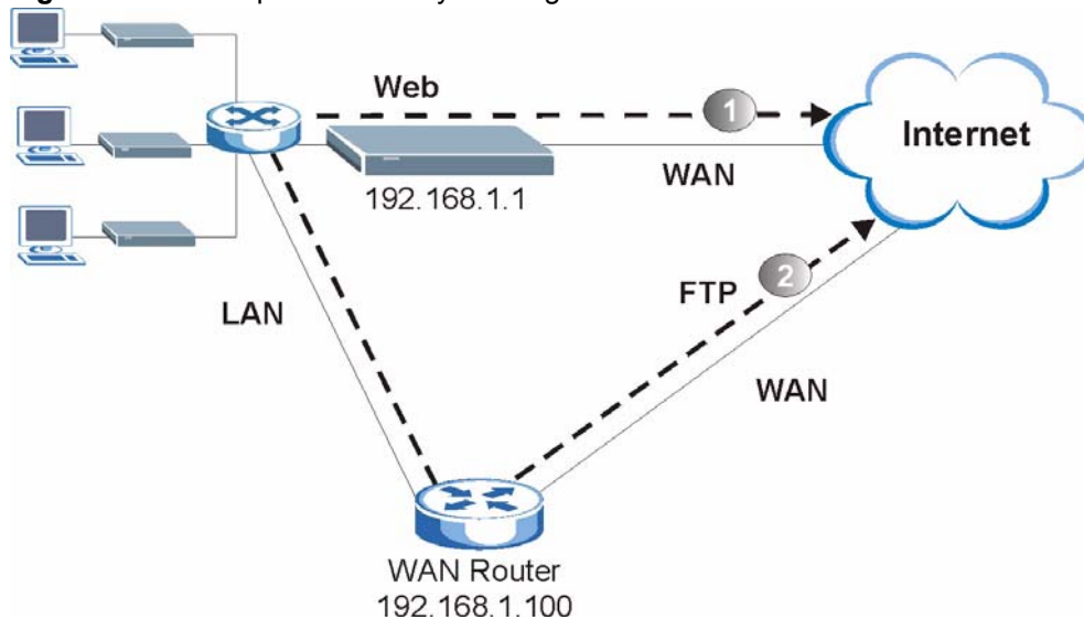
Figure 349 Example of IP Policy Routing
