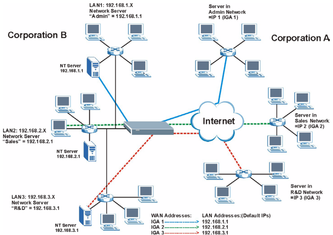
Figure 138 NAT Application With IP Alias
