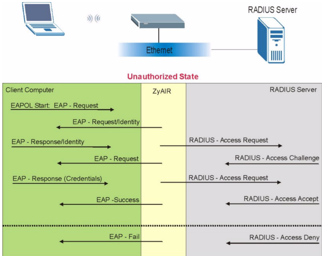
Figure 385 Sequences for EAP MD5–Challenge Authentication
