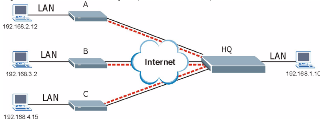
Figure 121 Telecommuters Using Unique VPN Rules Example
