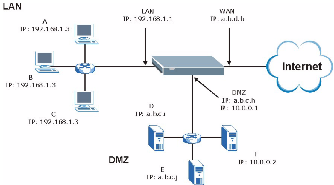
Figure 64 DMZ Private and Public Address Example
