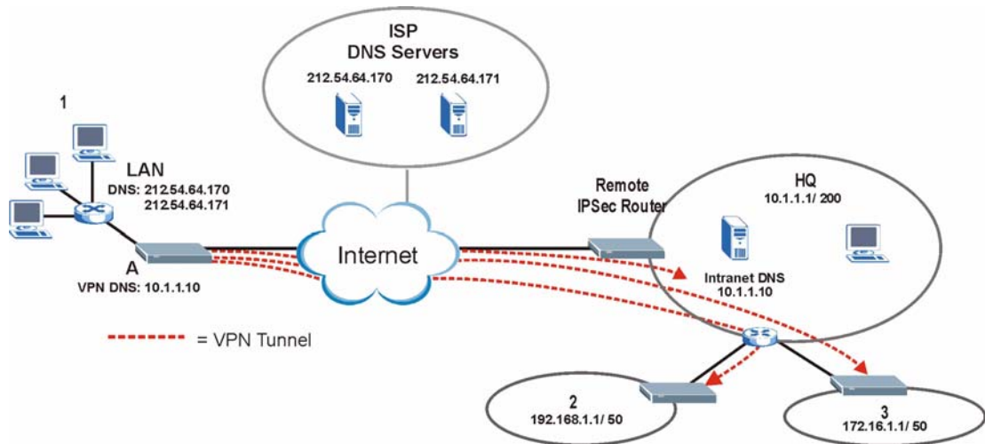
Figure 113 VPN Host using Intranet DNS Server Example
