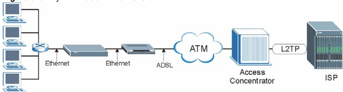
Figure 379 ZyWALL as a PPPoE Client
