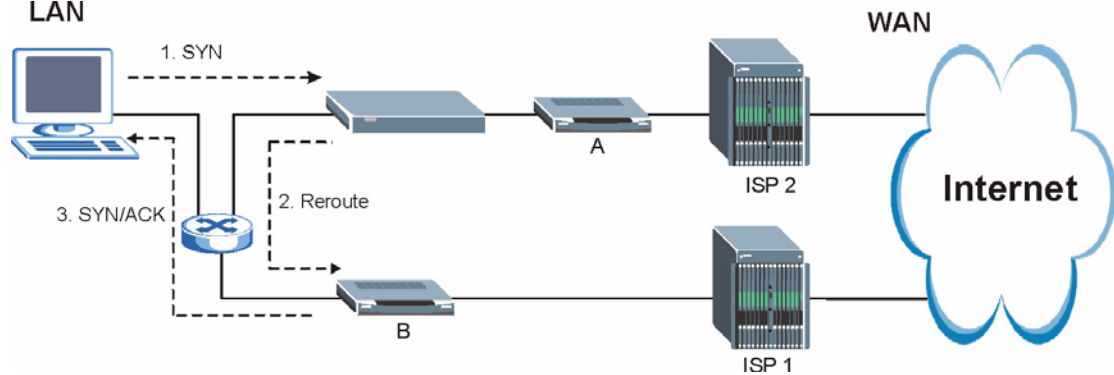
Figure 387 “Triangle Route” Problem LAN
