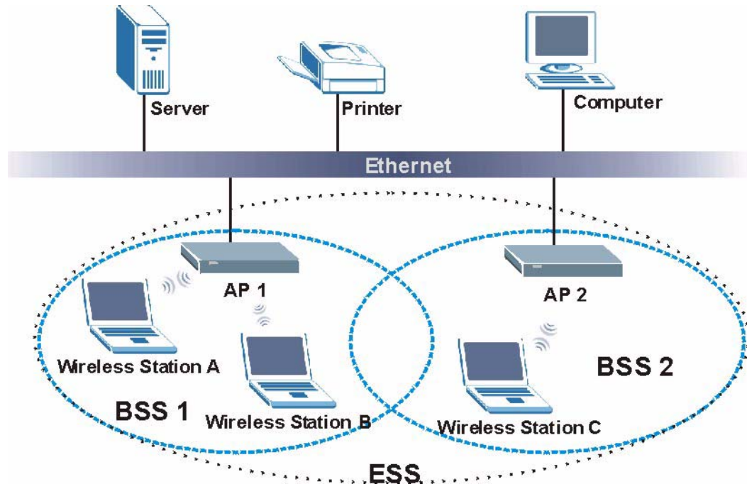
Figure 384 ESS Provides Campus-Wide Coverage
