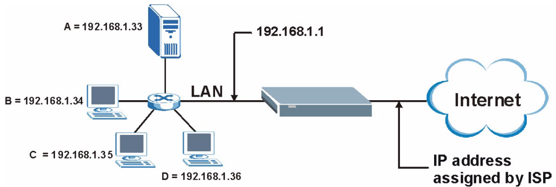
Figure 142 Multiple Servers Behind NAT Example
