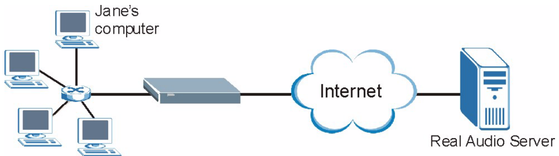
Figure 145 Trigger Port Forwarding Process: Example
