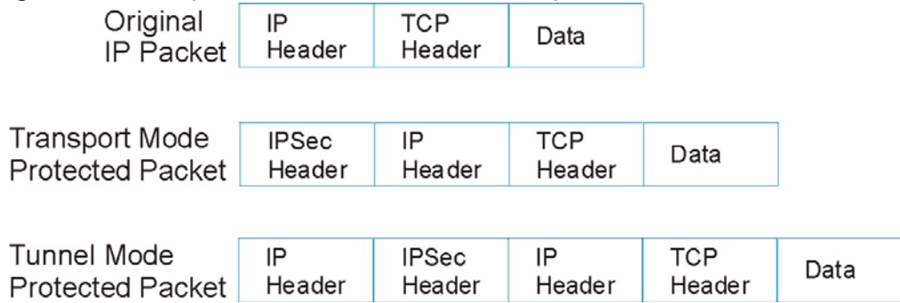
Figure 109 Transport and Tunnel Mode IPSec Encapsulation
