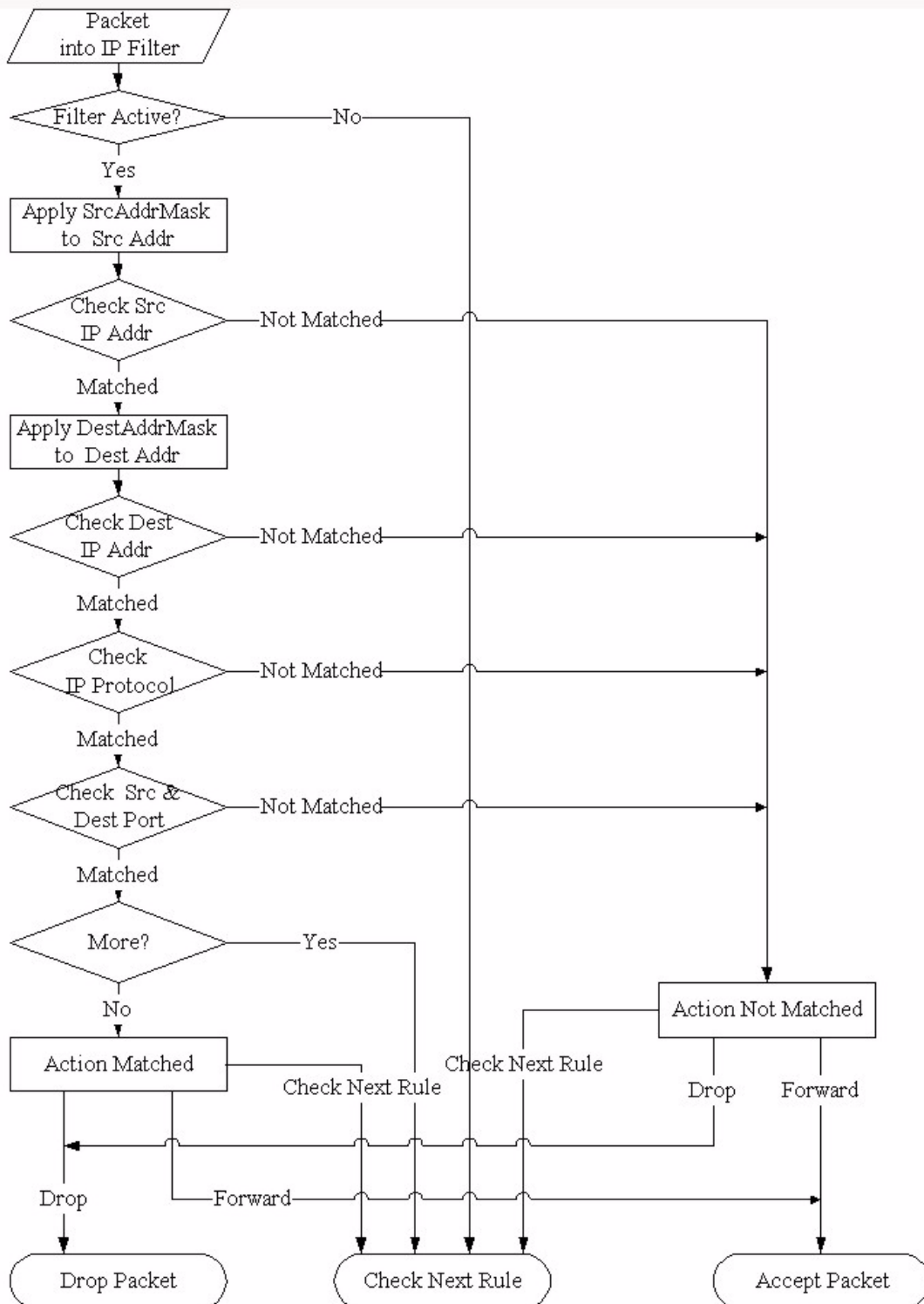
Figure 298 Executing an IP Filter
