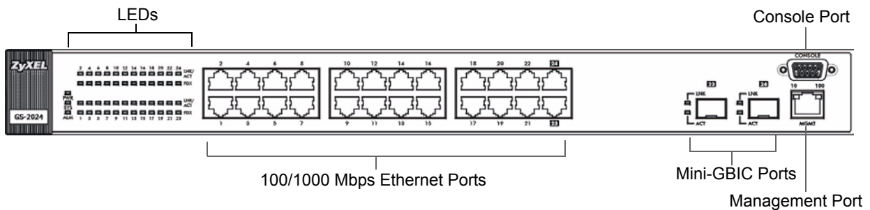
Figure 9 Front Panel
