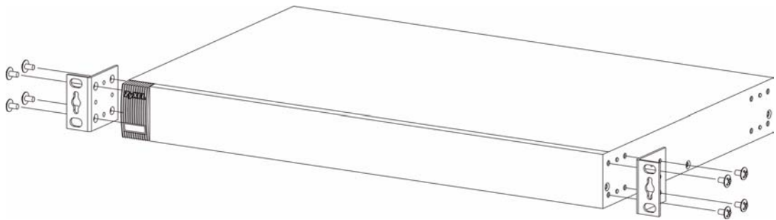
Figure 7 Attaching the Mounting Brackets
