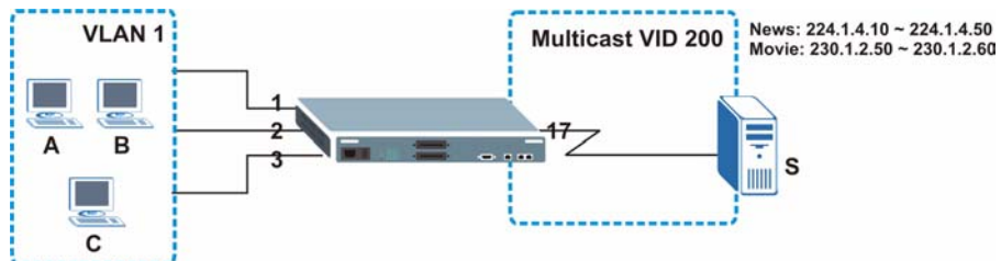
Figure 57 MVR Configuration Example
