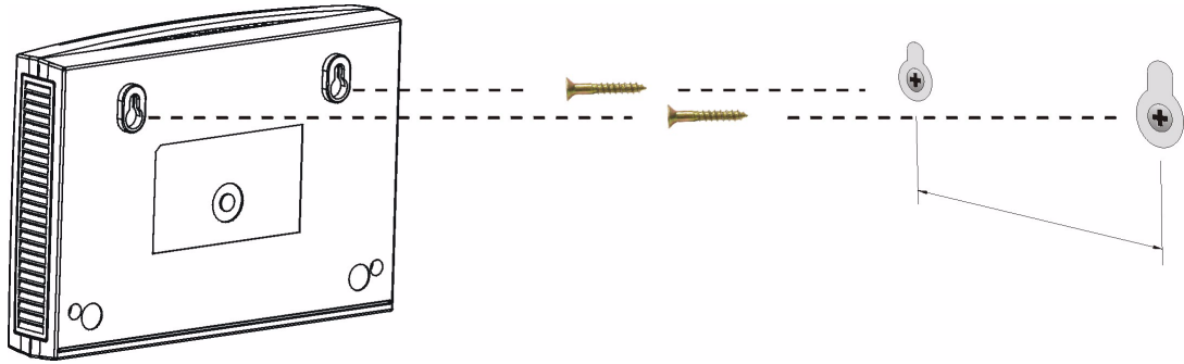
Figure 19 Wall-mounting Example
