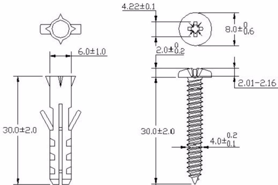
Figure 20 Masonry Plug and M4 Tap Screw
