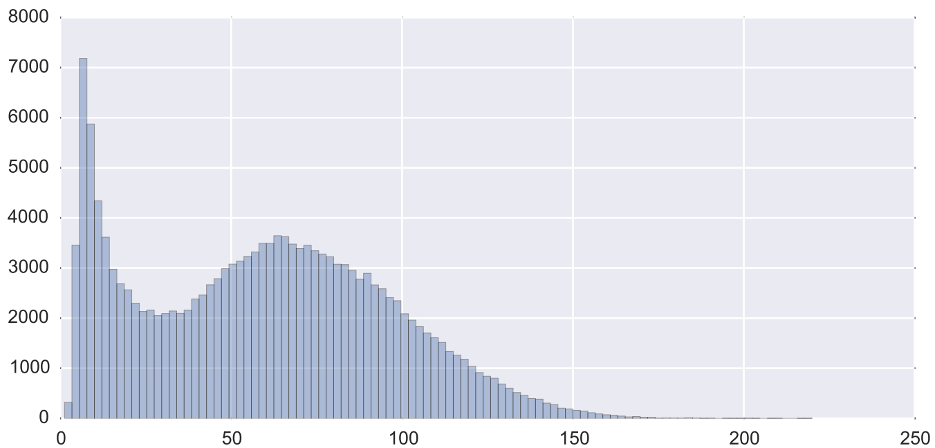
Subject 24772 tSNR inside the mask
