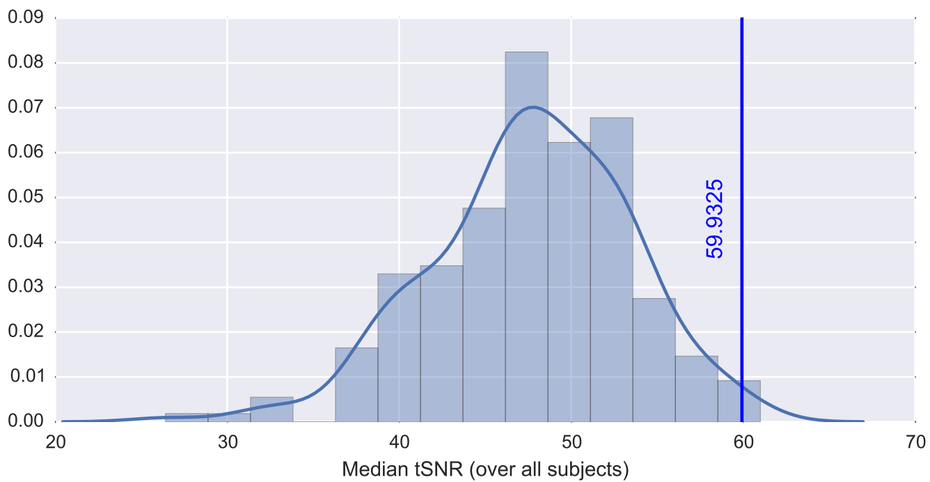
Subject 24772 tSNR inside the mask
